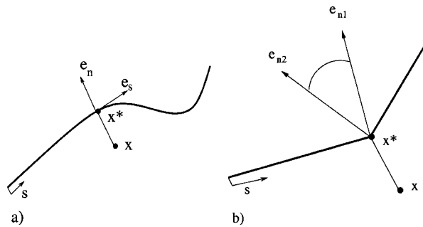
Figure 8. Illustration of normal and tangential co-ordinates for a smooth crack: (a) and for a crack with a kink; (b) x^* is the closest point to x on the crack. In both of the above cases, the jump function H(x) = -1
