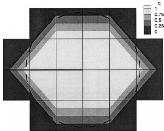
Figure 13. Weight function q on the elements
